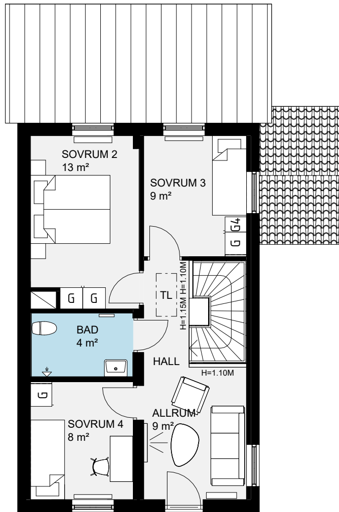
PLAN 2
